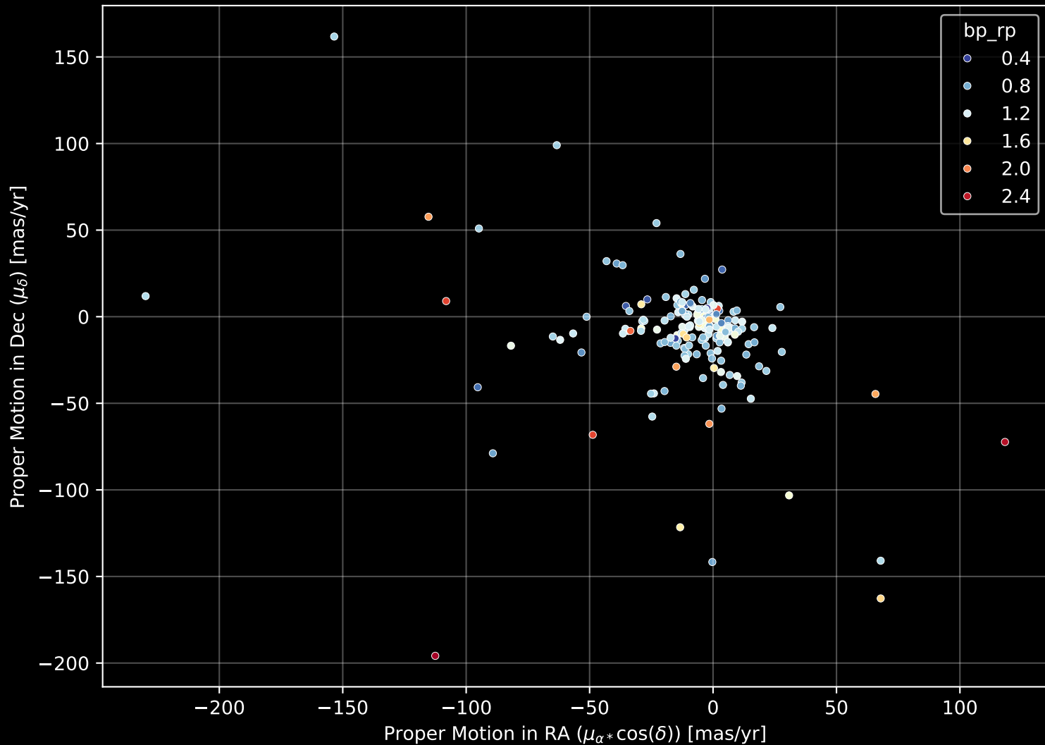
APOGEE DR17 Field: [020+43_MGA] Proper Motion Diagram (n= 195)
