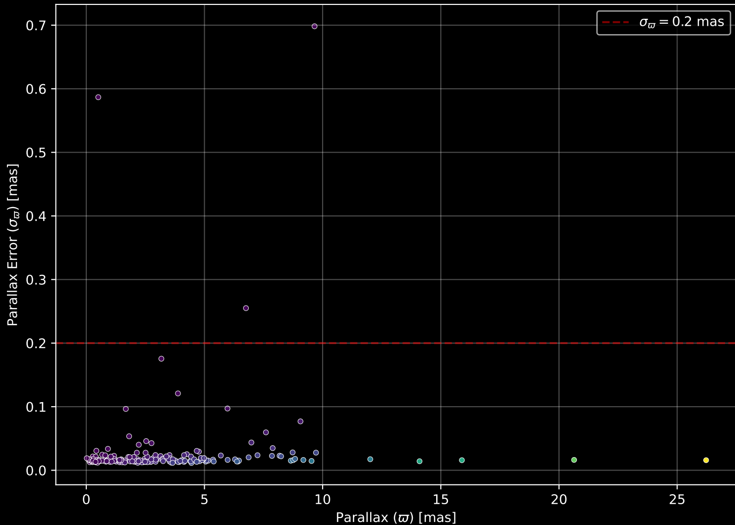
APOGEE DR17 Field: [020+43_MGA] Parallax Quality (n= 195)
