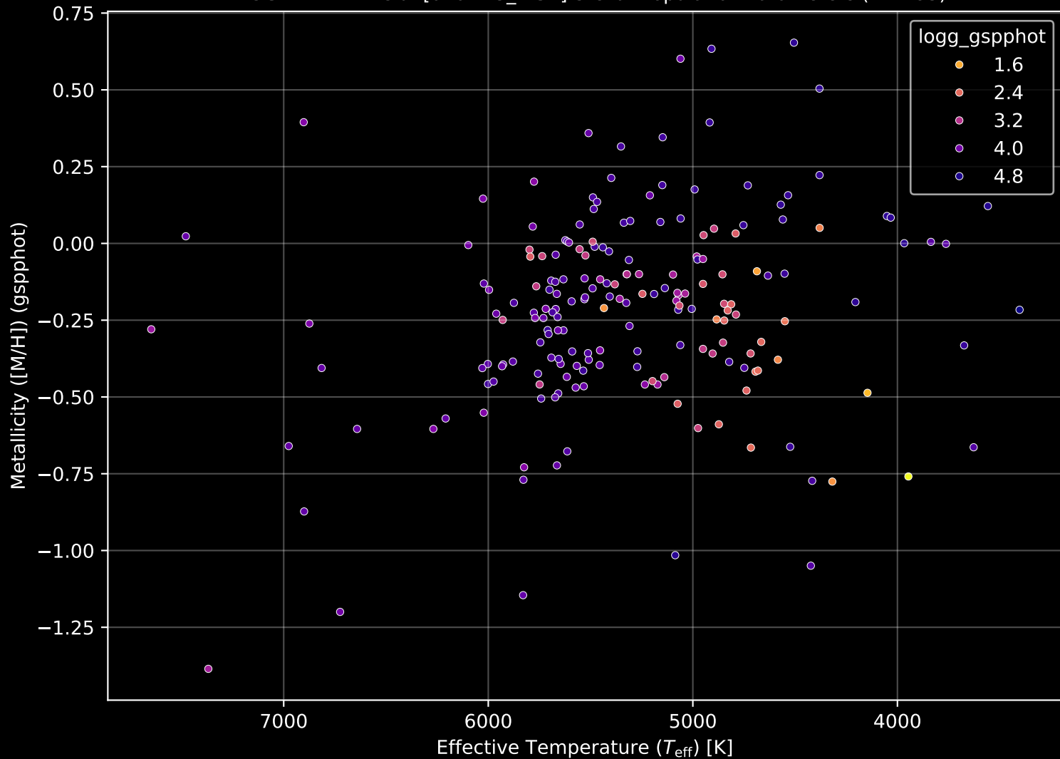
APOGEE DR17 Field: [020+43_MGA] Stellar Population Parameters (n= 195)
