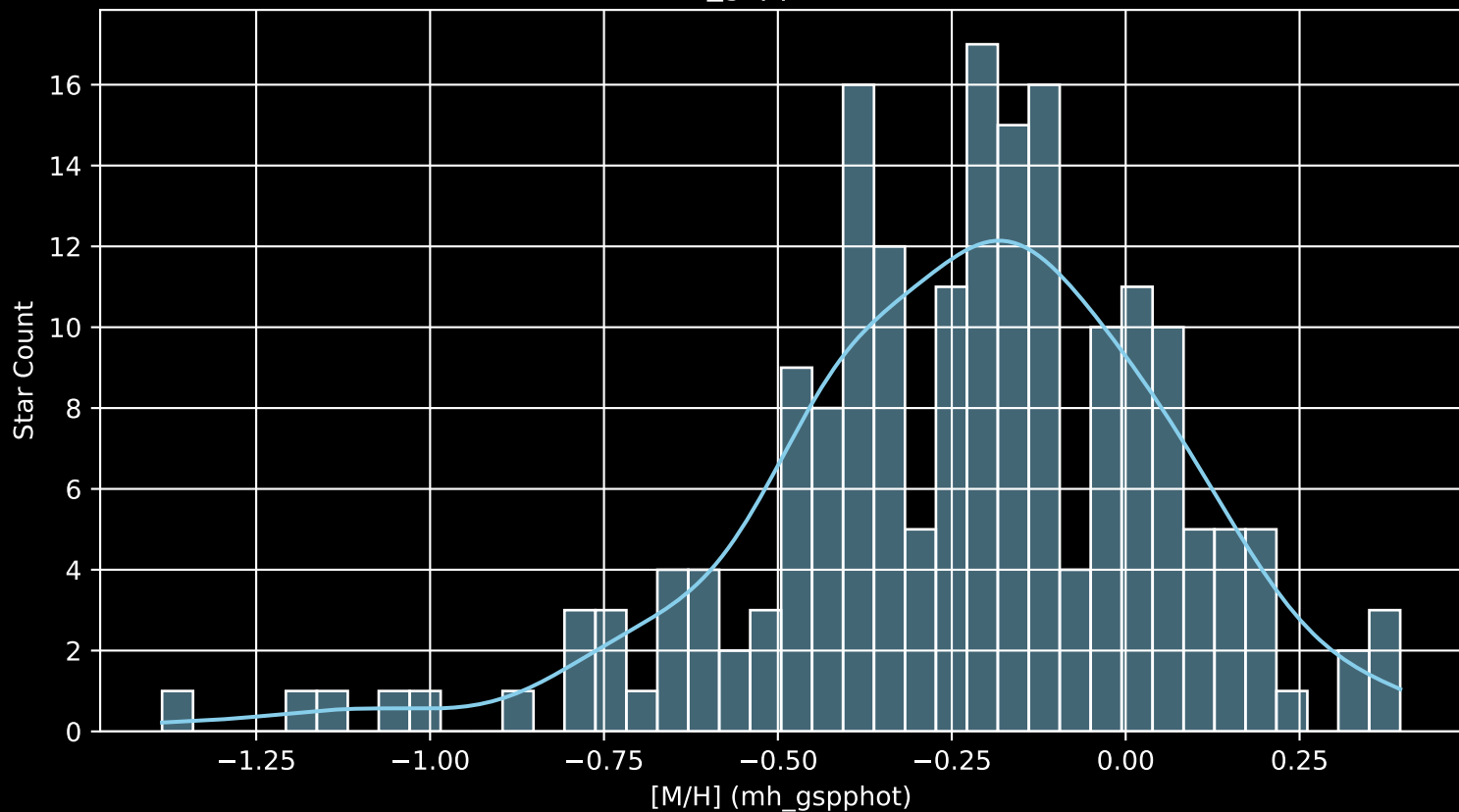
APOGEE DR17 Field: [020+43_MGA [M/H] (mh_gspphot) (n= 191)
