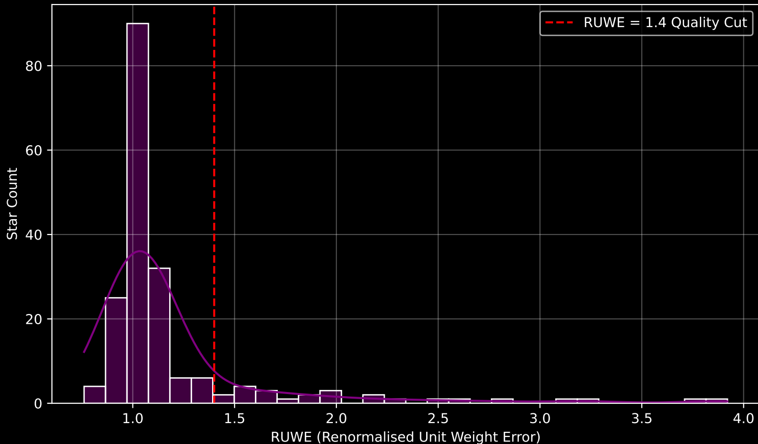
GAPOGEE DR17 Field [020+43_MGA] RUWE Distribution (n= 188)
