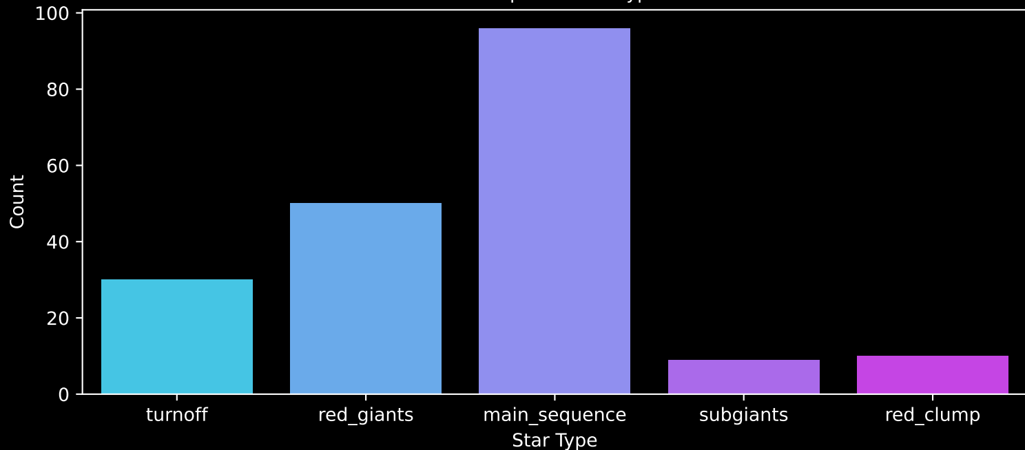
APOGEE DR17 Field: [020+43_MGA] Count plot of Star Type
